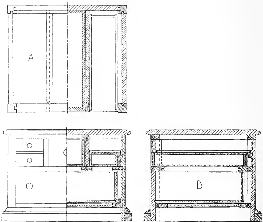
FIG. 455. COMMON TYPE OF CARCASE.
